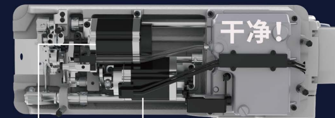
剪线马达 Auto-trimming 剪线&抬压脚马达 Auto-trimming & Auto-presser foot lifter motor
